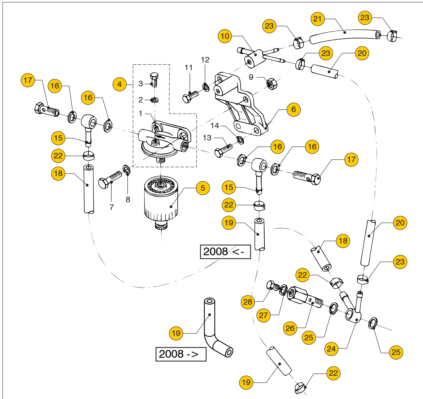
M2.02 M2.04 M2.06 M2.C5 Brandstofffilter 2014 <- M2.D5
