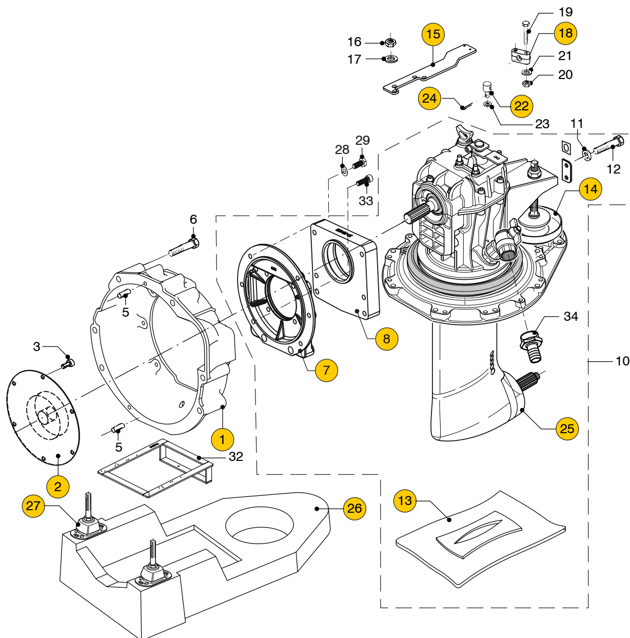
Saildrive ZF SD10 06-2020 ->
